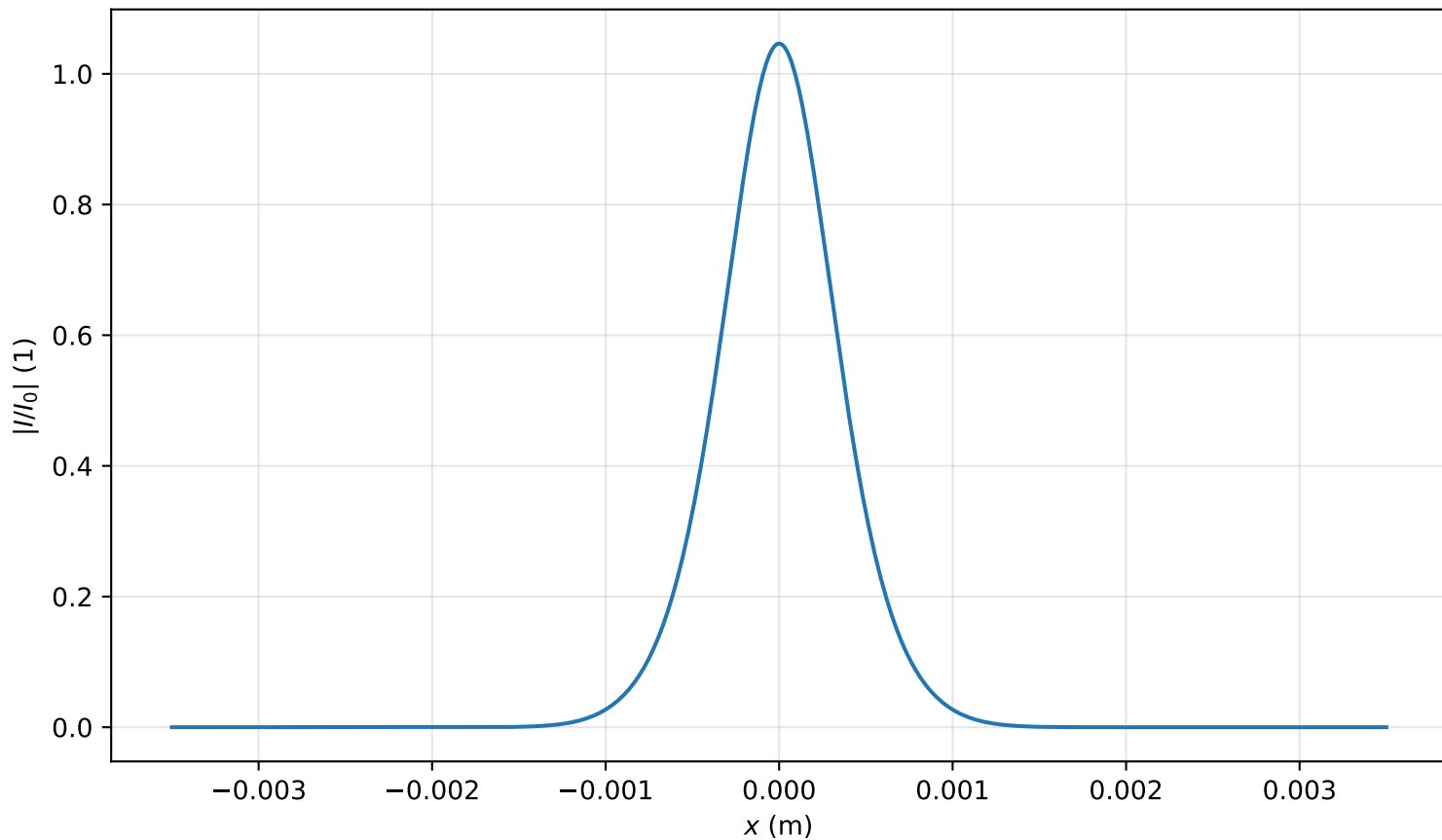
Intensity profile I(x, y = 0, z = 1.035m)/I_0 , P_{in}=0.5P_{cr} , artificial time
